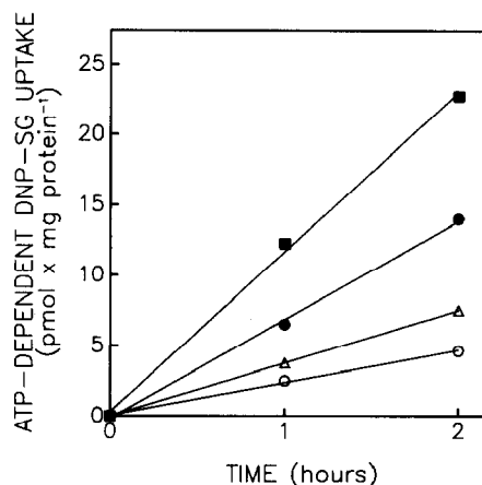
Fig. 1. Time course of S -dinitrophenylglutathione uptake by liver plasma membrane vesicles. Plasma membrane fraction ( \approx 70 \mu g protein/ml) was incubated at 37°C with 16 \mu M DNP-SG in Tris-HCl buffer, pH 7.4, supplemented with 1 mM EGTA, 1 mM ouabain and 180 mM sucrose. Uptake of DNP-SG was determined as described in section 2. (○) In the absence of ATP and Mg^{2+} , (Δ) plus 2 mM Mg^{2+} , (●) plus 2 mM Tris-ATP, (■) plus 2 mM Mg^{2+} and 2 mM Tris-ATP. One experiment typical of four.
